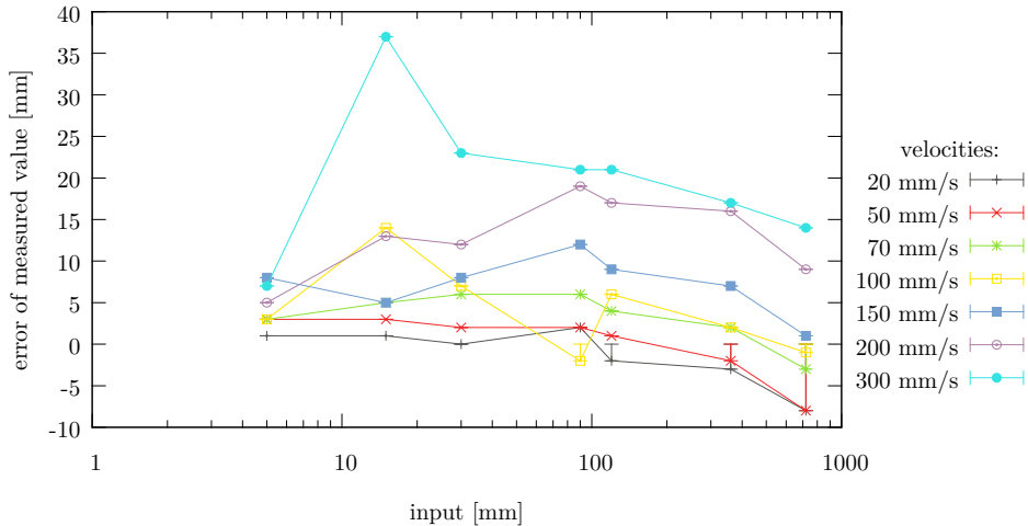
Soft Start/Stop, laminate floor, turn on spot
