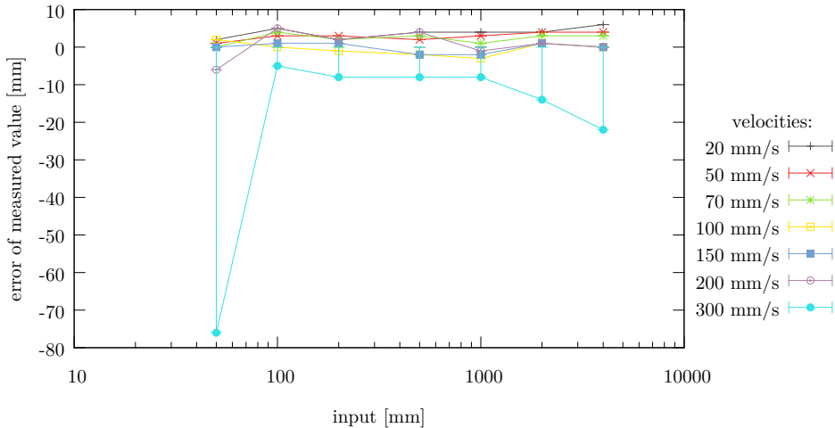
Arithmetic Mean Correction, laminate floor, straight drive
