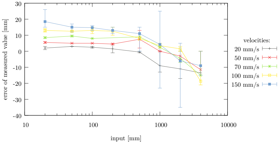
Original behaviour, carpet floor, straight drive
