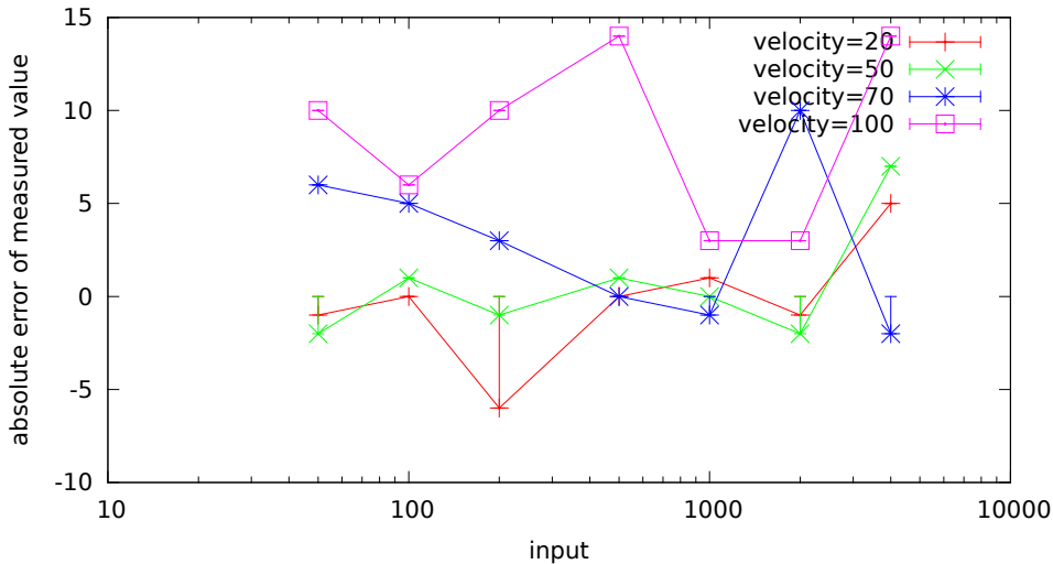
Arithmetic Mean Correction, carpet floor, straight drive
