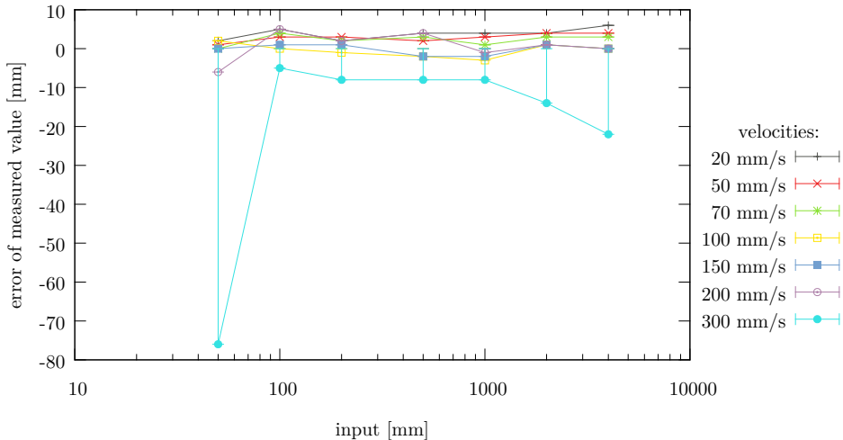
Arithmetic Mean Correction, laminate floor, straight drive
