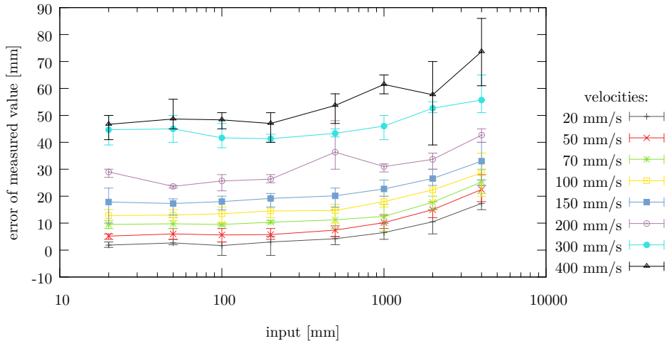
Original behaviour, laminate floor, straight drive
